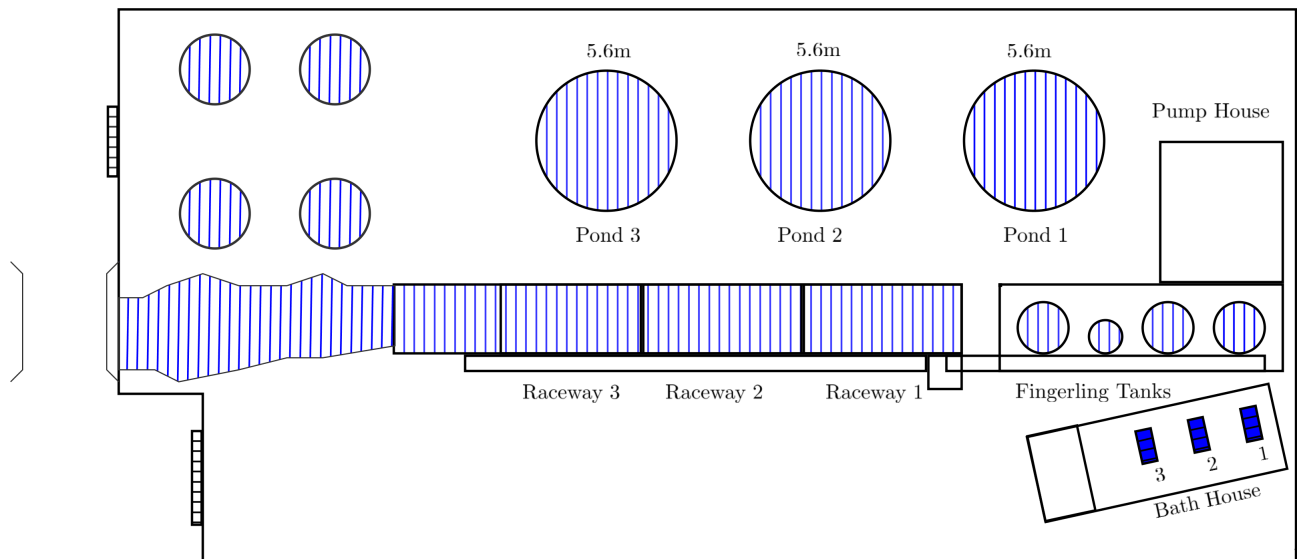
Figure 2.1: Mbona Hatcheries Layout.
